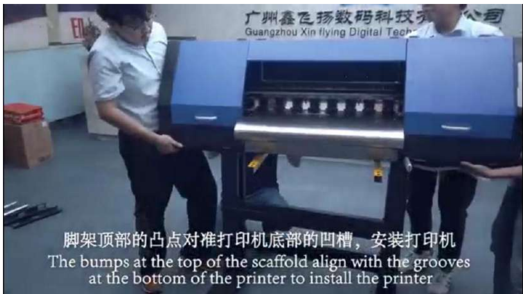
脚架顶部的凸点对准打印机底部的凹槽，安装打印机 The bumps at the top of the scaffold align with the grooves at the bottom of the printer to install the printer
